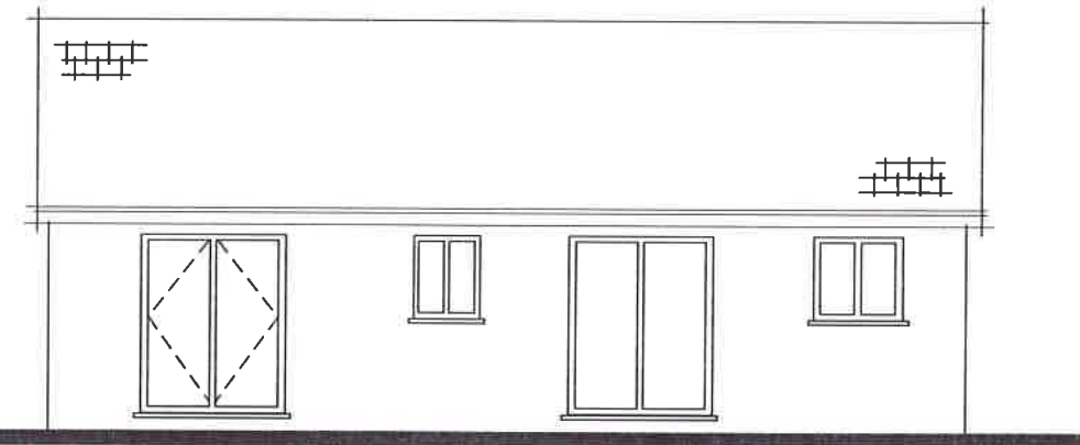
EXISTING REAR ELEVATION (NORTH)
